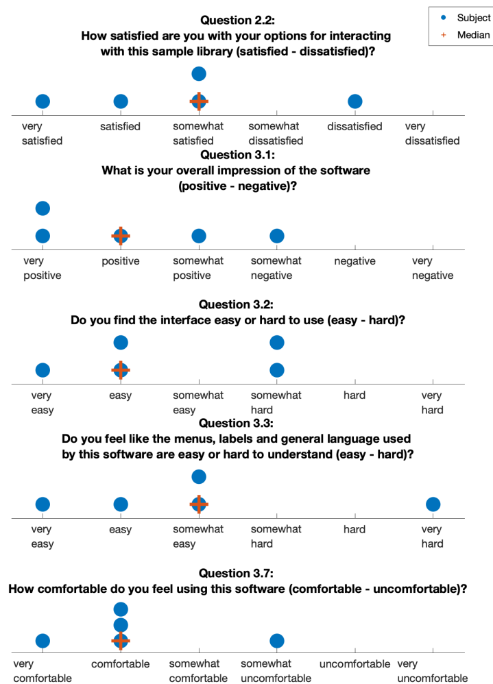
Figure 16: Likert scale ratings by interview subjects for questions concerning satisfaction with their current sample library workflow and first SOM Browser impressions
