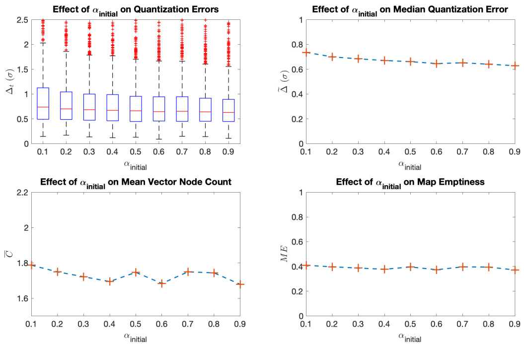
Figure 9: SOM Browser : effect of \alpha_{initial} on SOM metrics. SOM parameters: mapSize = 32 \times 32 , training duration = 10^4 steps, linearly decreasing \alpha with \alpha_{initial} = [0.9, \dots, 0.1] , r_{start} = 6.4 , r_{end} = 1
